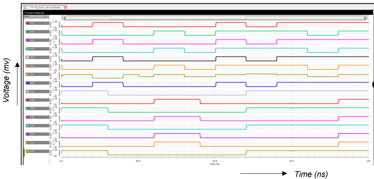
Fig: 4.11: 6T SRAM Macro Output Waveforms
