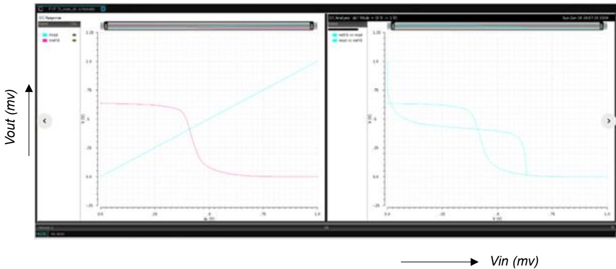
Fig: 4.14: DC Analysis – 7T SRAM
