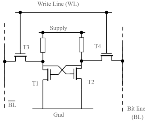
Fig:1.1 Typical SRAM Cell Structure (Ref: [31])
