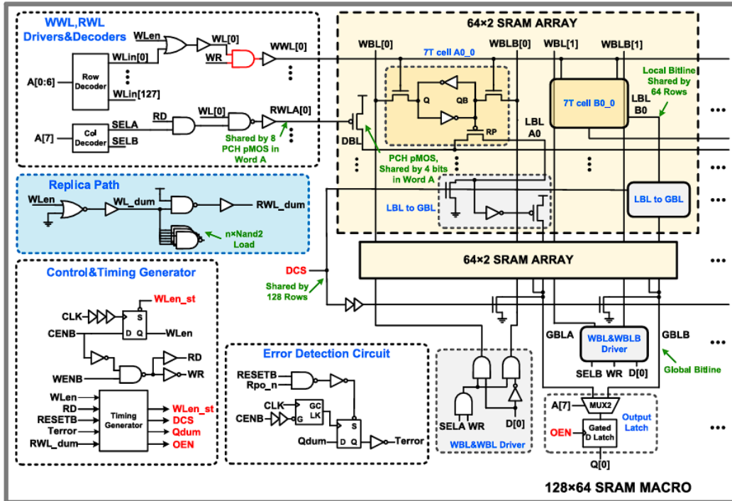
Fig. 3.1: Existing 128×64 SRAM macro with 7T SRAM cell. (Ref – [11])
