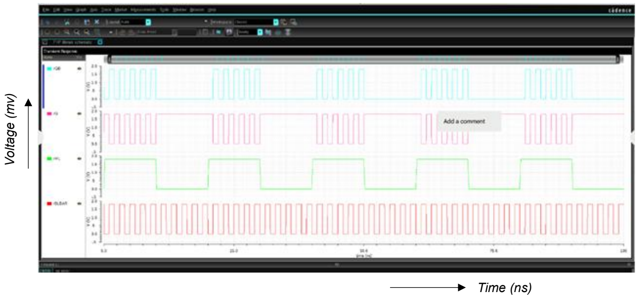
Fig: 4.9: Transient Analysis – 6T SRAM
