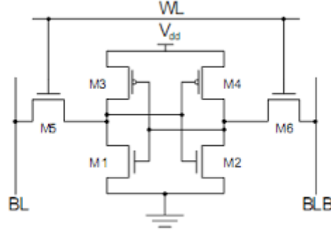
Fig: 4.1: Conventional 6T SRAM Cell Architecture
